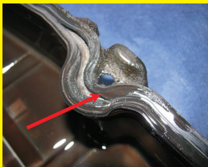
Split gasket caused by over torquing
